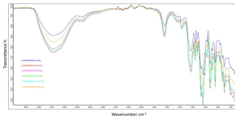
Figure 2. FTIR spectras of carrageenan after treated with gamma ray at various doses
