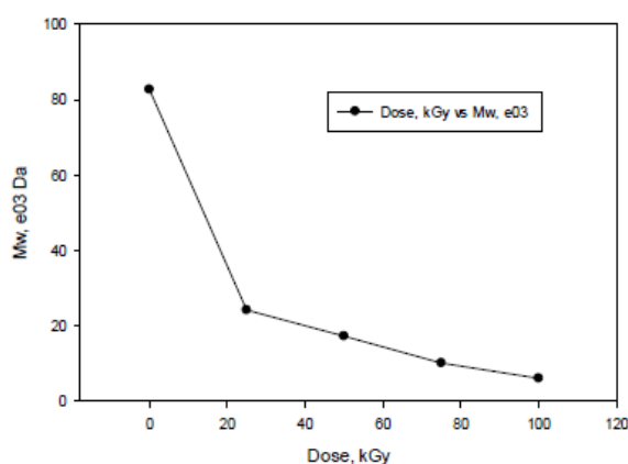
Figure 1; Effect of absorbed dose on Mw of carrageenan.
