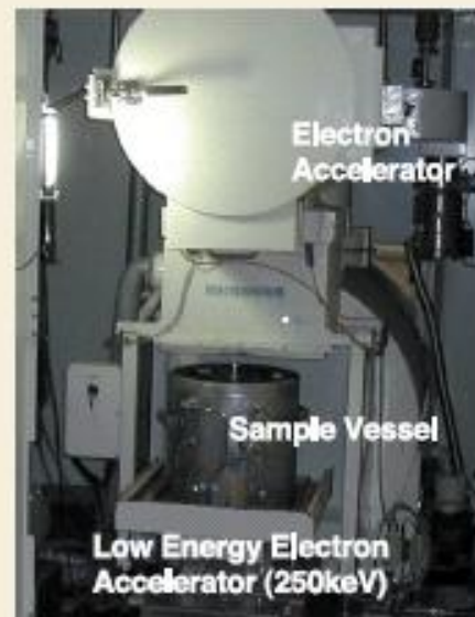
Radiation Decomposition of Natural Polymer in Water
